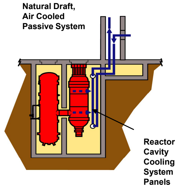
B) Passive Reactor Cavity Cooling System
